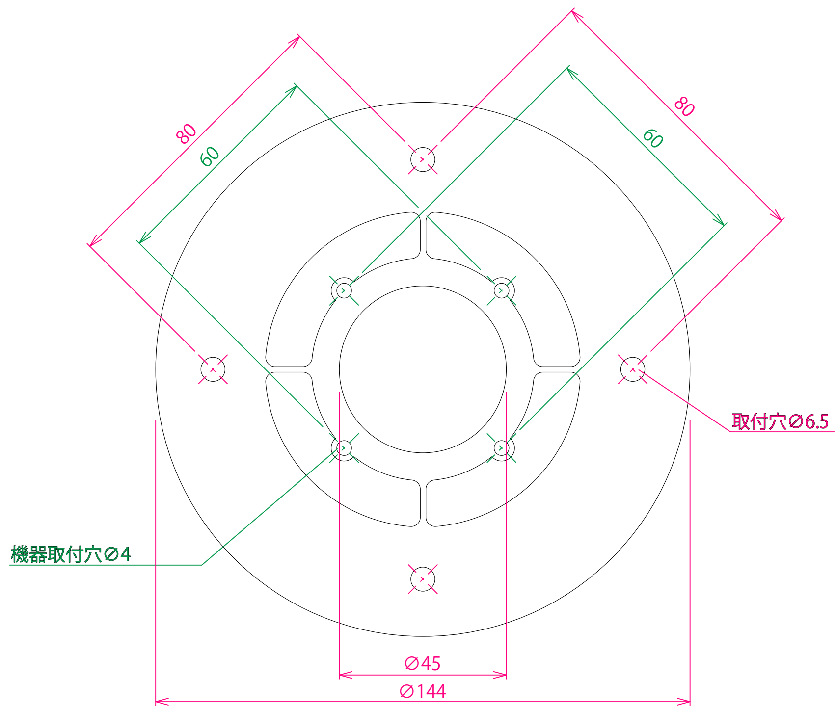
Cover disc
